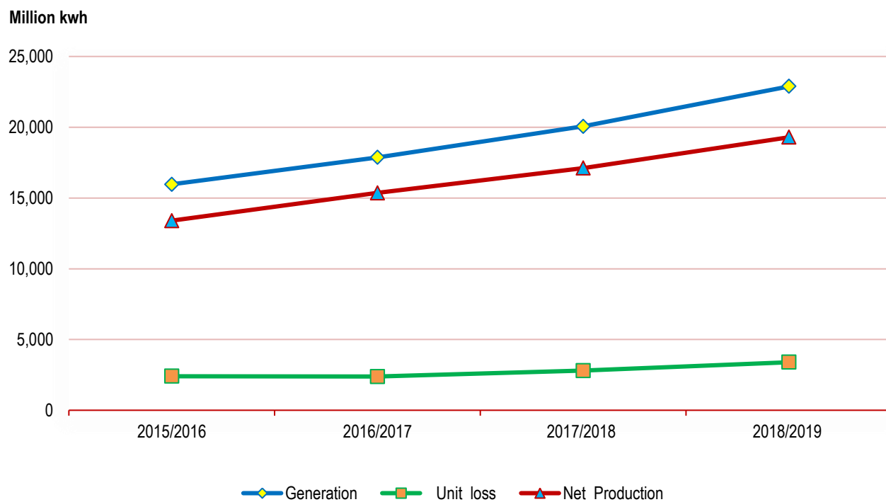
FIGURE 11.5 PRODUCTION OF ELECTRIC POWER
